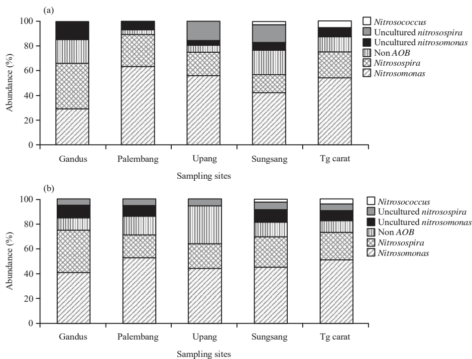
Fig. 2(a-b): AOB abundance based on T-RFLP analysis derived from (a) amoA gene in the rainy season and (b) amoA gene in the dry season
