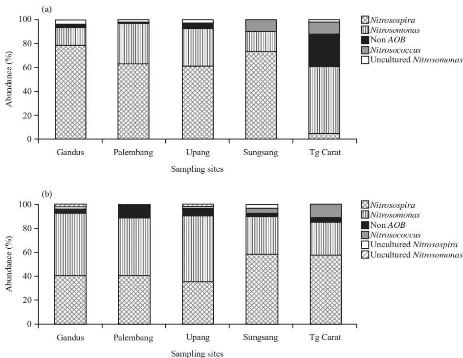
Fig. 1(a-b): AOB abundance based on T-RFLP analysis derived from (a) 16S rRNA gene in the rainy season and (b) 16S rRNA gene in the dry season Freshwater sites: Gandus, Palembang, and Upang. Brackish water sites: Sungsang and Tg Carat
