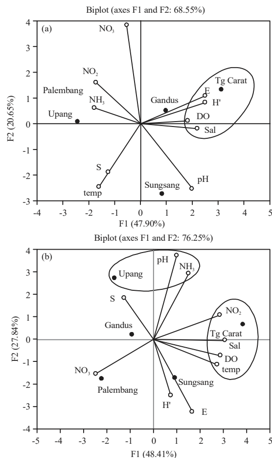
Fig. 4(a-b): PCA of relationship between AOB community and physicochemical properties to sampling sites derived from (a) amoA gene in the rainy season and (b) amoA gene in the dry season
