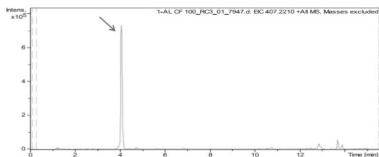
Fig. 3. Chromatogram of Lincomycin
