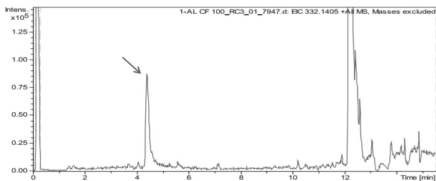
Fig. 2. Chromatogram of Ciprofloxacin
