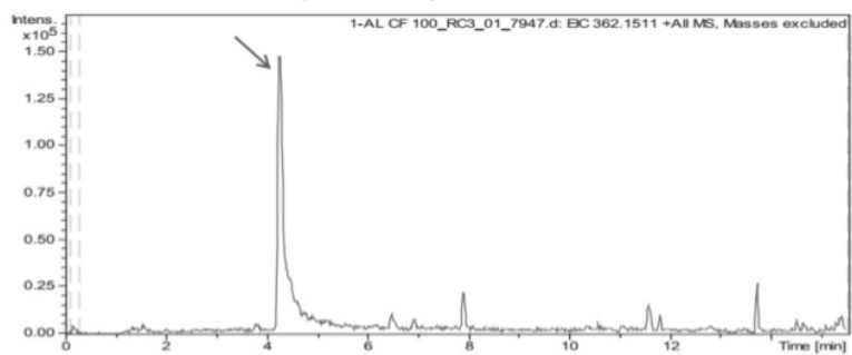
Fig. 6. Chromatogram of Ofloxacin/Levofloxacin
