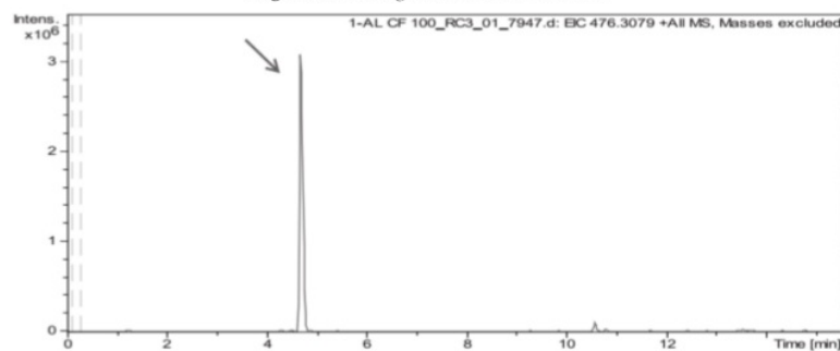
Fig. 5. Chromatogram of Netilmicin
