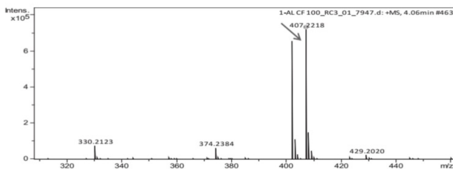
Fig. 8. Spectrum of Lincomycin
