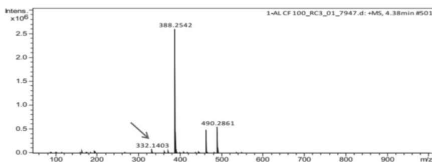
Fig. 7. Spectrum of Ciprofloxacin
