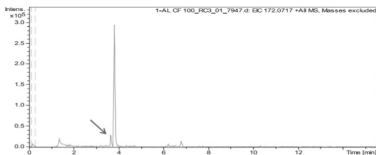
Fig. 4. Chromatogram of Metronidazole
