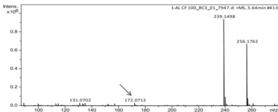
Fig. 9. Spectrum of Metronidazole
