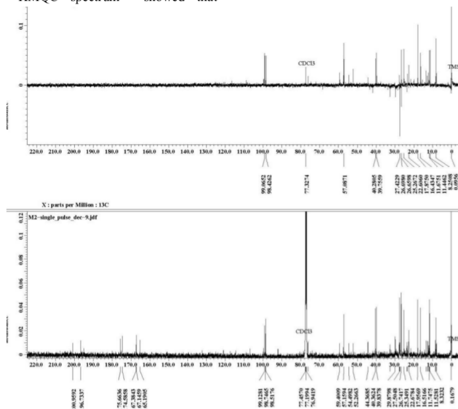
Figure 2. ^{13}\text{C} NMR spectrum isolated compound
