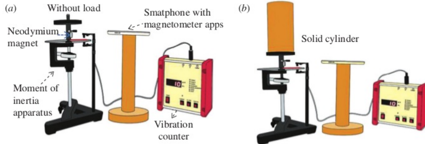
Figure 1. Schematic of the MOI analysis using a smartphone magnetometer. (a) Without load, and (b) with solid cylinder.
