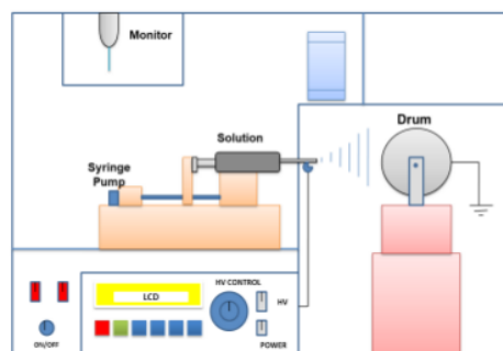
Figure 1. Electrospinning setup
