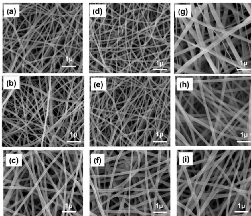
Figure 2 Scanning Electron Microscopic observation at massa rasio with variation of (a-c) flow rate (0.1 mL/h, 0.5 mL/h, 1 mL/h), (d-f) voltage (10 kV, 14 kV, 18 kV) and (g-i) TCD (8 cm, 12 cm, 16 cm)
