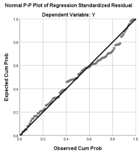
Gambar 4.2 Normal Probability Plot (Model Regresi II)
