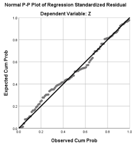
Gambar 4.1 Normal Probability Plot (Model Regresi I)
