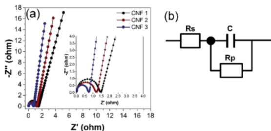
Fig. 12 (a) Nyquist plots of the electrospun composite nanofibers. Inset: magnification of the region between 0.0 and 4.0 \Omega . (b) Equivalent circuit diagram derived from the Nyquist plots.
