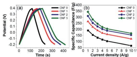
Fig. 11 (a) CGD profiles of the mats at a current density of 2 \text{ A g}^{-1} . (b) Specific capacitance values of the composite fiber mat electrodes at various current densities.
