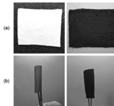
Fig. 4 Photographs of (a) PAN and PAN/rGOPKS mats and (b) electrodes.
