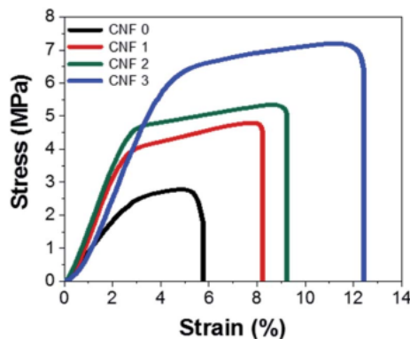
Fig. 9 Stress-strain curves of the fibrous mats.
