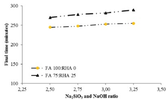
FIGURE 6. The effect of \text{Na}_2\text{SiO}_3 and NaOH ratio on final setting time test result
