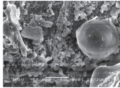
(b) \text{Na}_2\text{SiO}_3/\text{NaOH} 2.75
