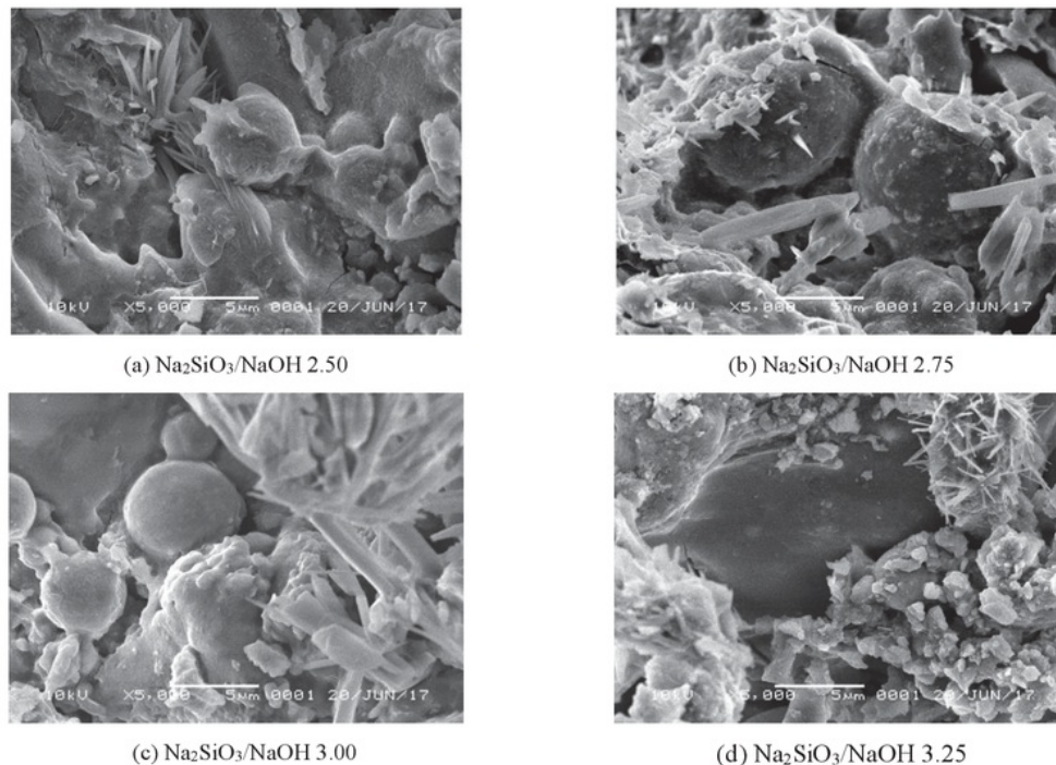
FIGURE 15. The result of SEM FA 50: RHA 50
