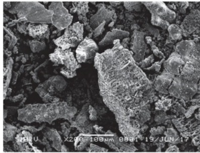
FIGURE 2. SEM microstructure of RHA
