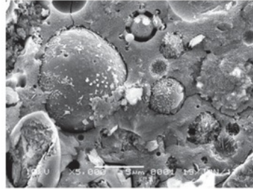
(b) \text{Na}_2\text{SiO}_3/\text{NaOH} 2.75
