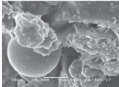
(c) \text{Na}_2\text{SiO}_3/\text{NaOH} 3.00
