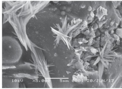
(a) \text{Na}_2\text{SiO}_3/\text{NaOH} 2.50
