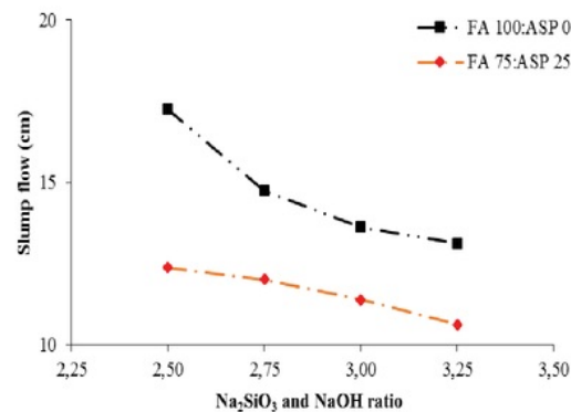
FIGURE 3. The effect of \text{Na}_2\text{SiO}_3 and NaOH ratio on slump flow test result
