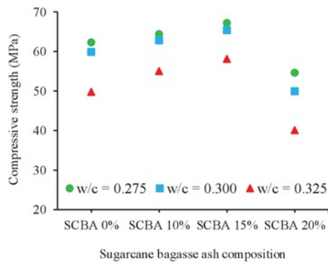
FIGURE 11. The effect of sugarcane bagasse ash composition on concrete compressive strength on age 28 days
