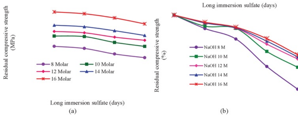
FIGURE 6. Compressive strength after immerse in sulfate
