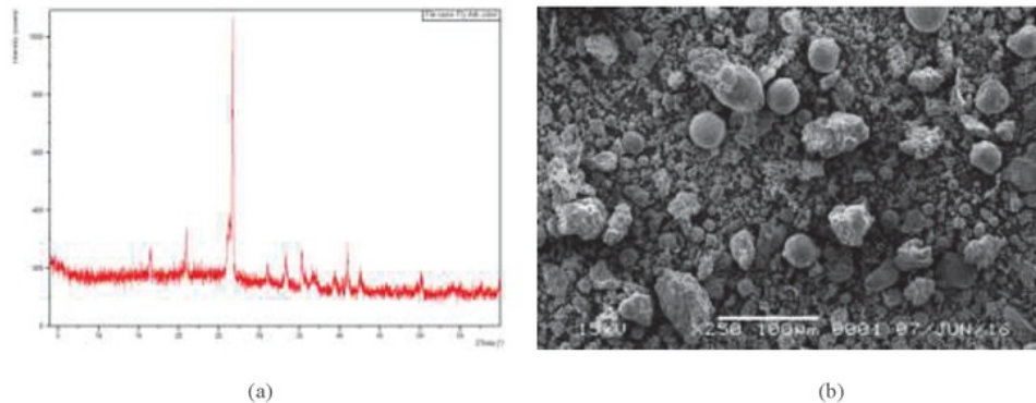
FIGURE 1. Characteristic of fly ash (a) The result of XRD test of fly ash (b) The SEM of fly ash
