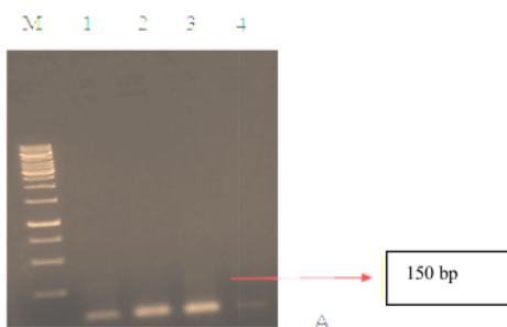
Figure 3. The result of electrophoresis with 1% gel agarose gel PCR Thrips in pairs primer ITS 2, row 1 ( long T. parvispinus , 2 ( medium T. parvispinus , 3 ( short T. parvispinus ): amplified, and 4 (male individu) : not amplified, row M: marker 100 bp (Sigma).
