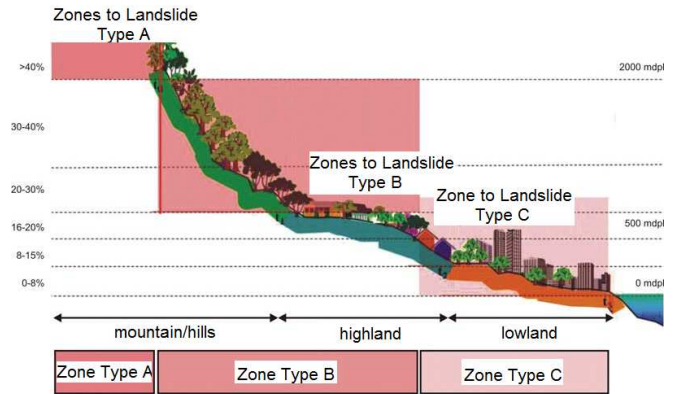
Fig. 2 Typology of the potential landslide zone
