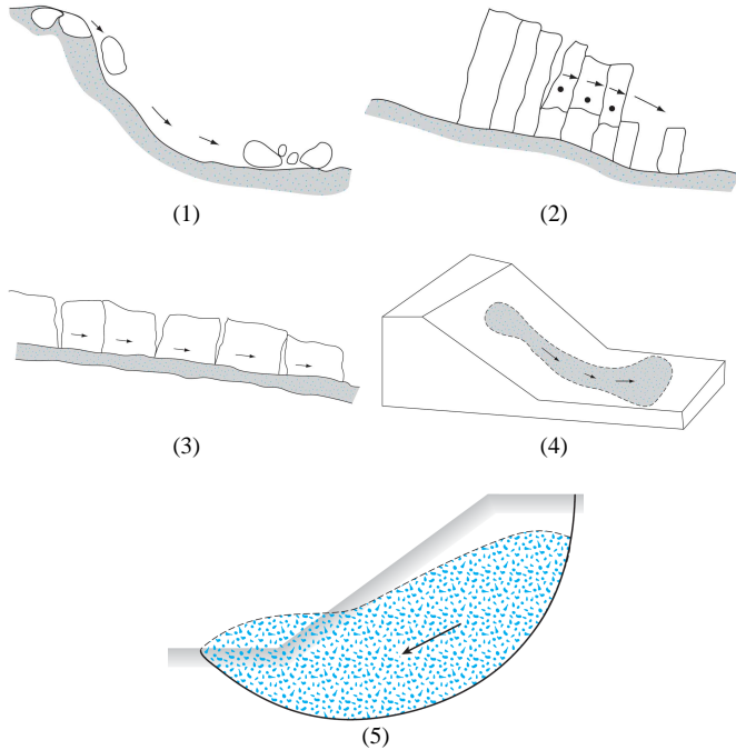
Fig. 1 Type of landslide
