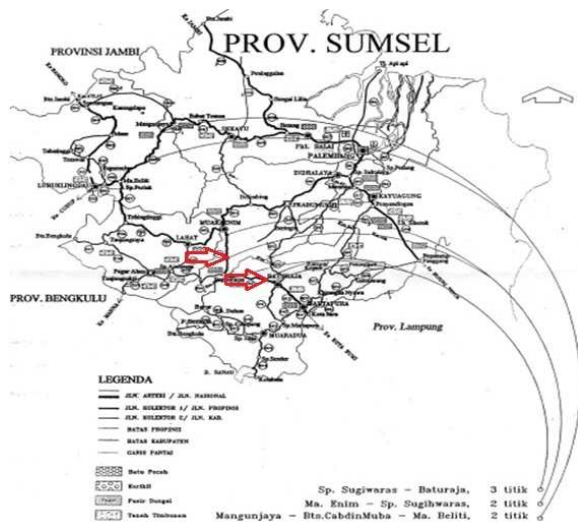
Fig. 3 Landslide location in Muara Enim Regency
