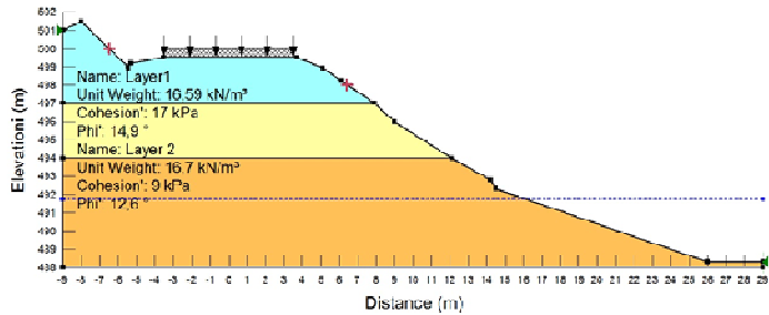
Fig. 4 Cross section in case study SP. Sugihwaras-Baturaja
