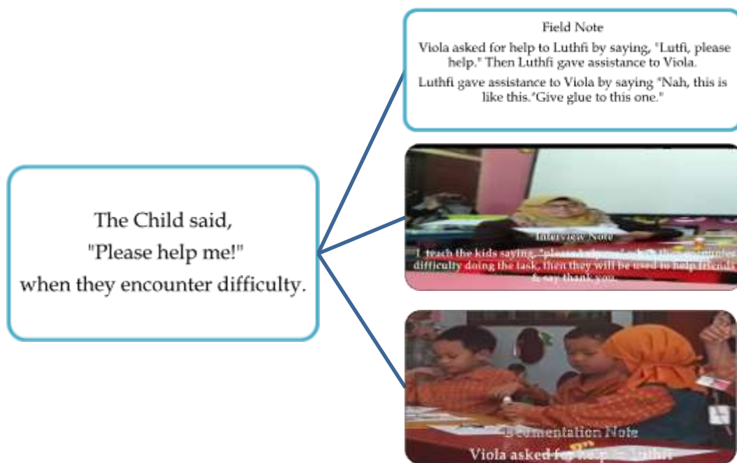
Chart 1. Display Data
