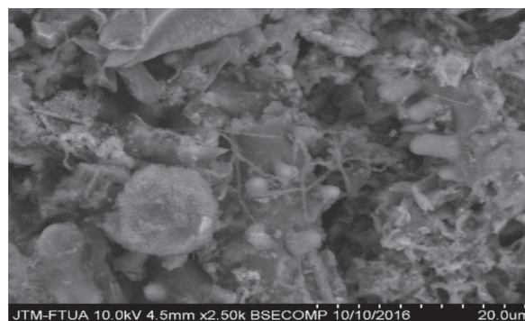
Fig. 2. The SEM image of husk Biochar.
