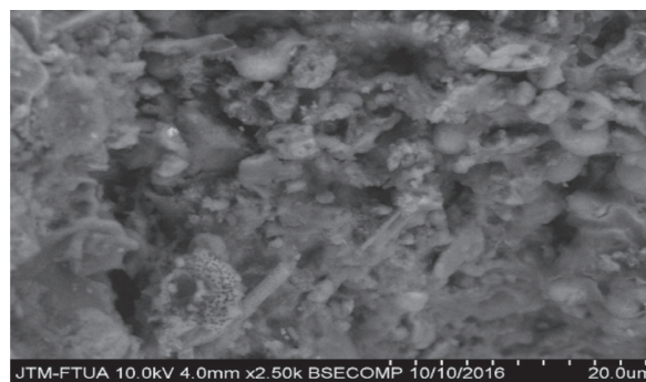
Fig. 3. The SEM image of straw compost
