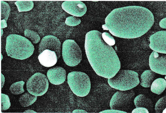
Pati ganyong HMT 80° C, 8 jam, GX 0% , 500x
