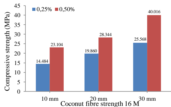
Fig 4. Fibre Length and Compressive Strength 16M
