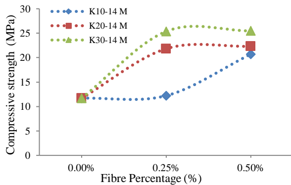
Fig 1. Fibre (%) and Compressive Strength 14M 16M
