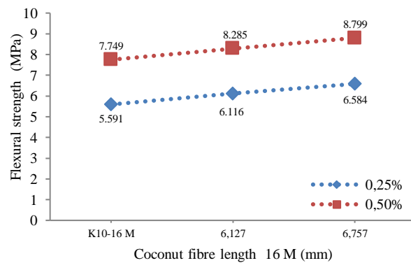
Fig 9. Fibre and Flexural Strength 16M
