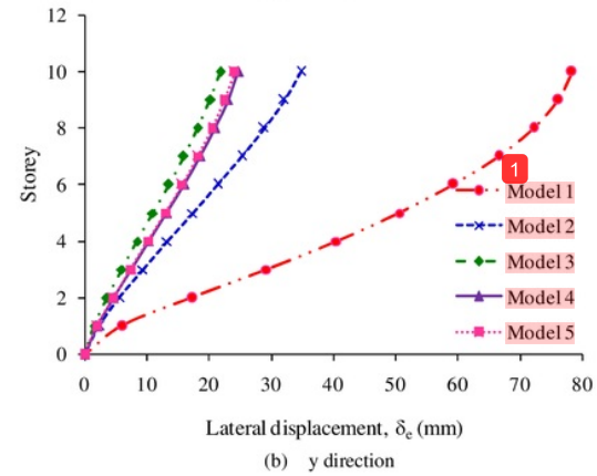
Fig. 5 Lateral displacements
