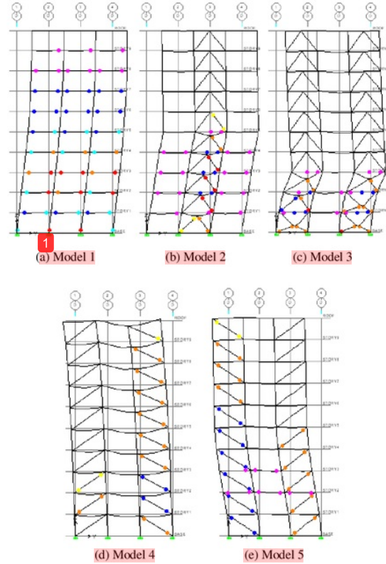
Fig. 11. The plastic hinges in the last step for earthquake in y direction
