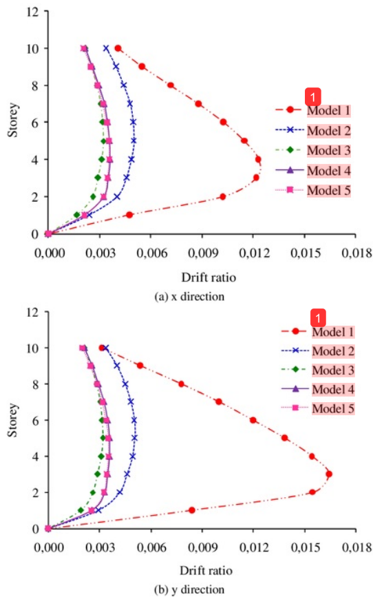
Fig. 6 Drift ratio
