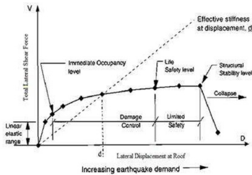
Fig. 1 Pushover curve (ATC-40)
