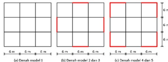
Fig. 2 Building layout
