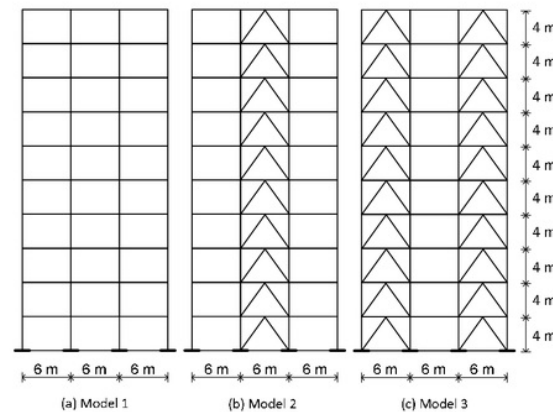
Fig. 2 Building layout
