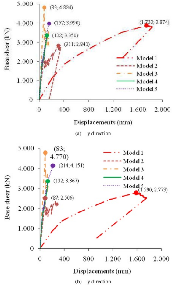
Fig. 7 Capacity curve
