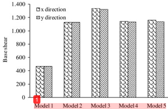
Fig. 4 Base shear (kN)
