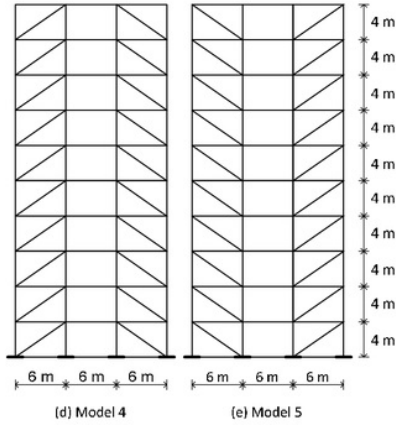
Fig. 3 Structure models
