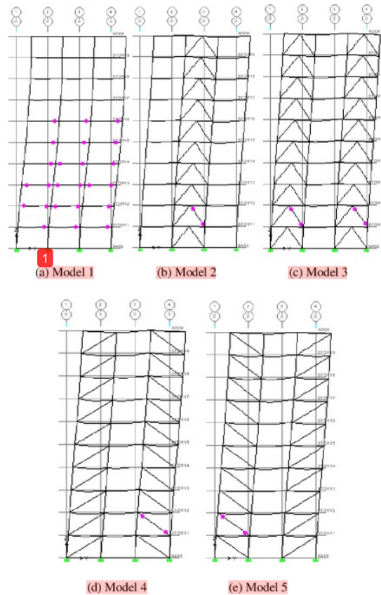
Fig. 9 The plastic hinges in the first step for earthquake in y direction
