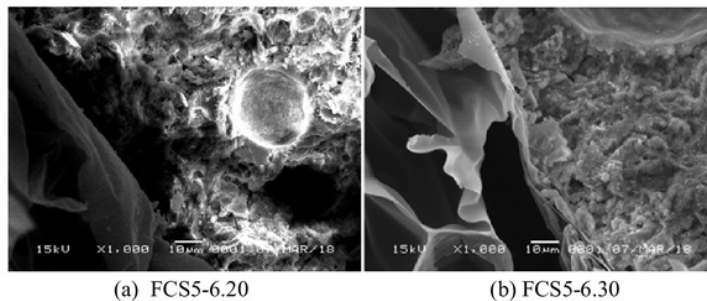
Figure 6. SEM photo of 5-6 mm styrofoam's diameter
