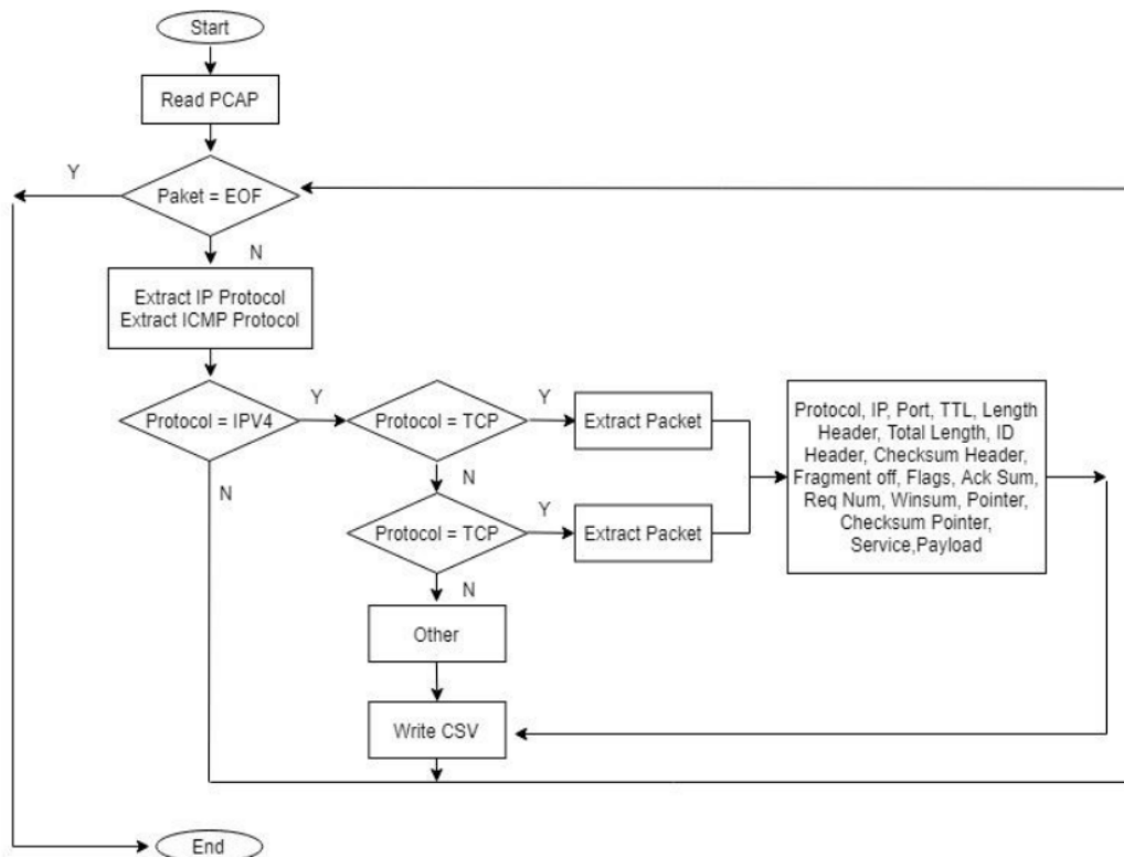
Figure 3. Feature Extraction Process
