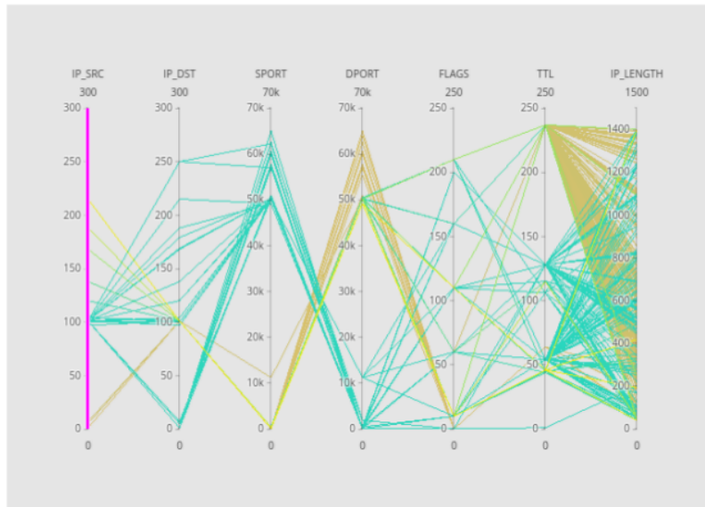
Figure 8. Multiraid Traffic Pattern Visualization
