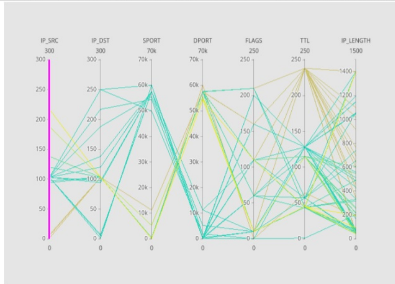
Figure 6. Solo Raid Pattern Visualization
