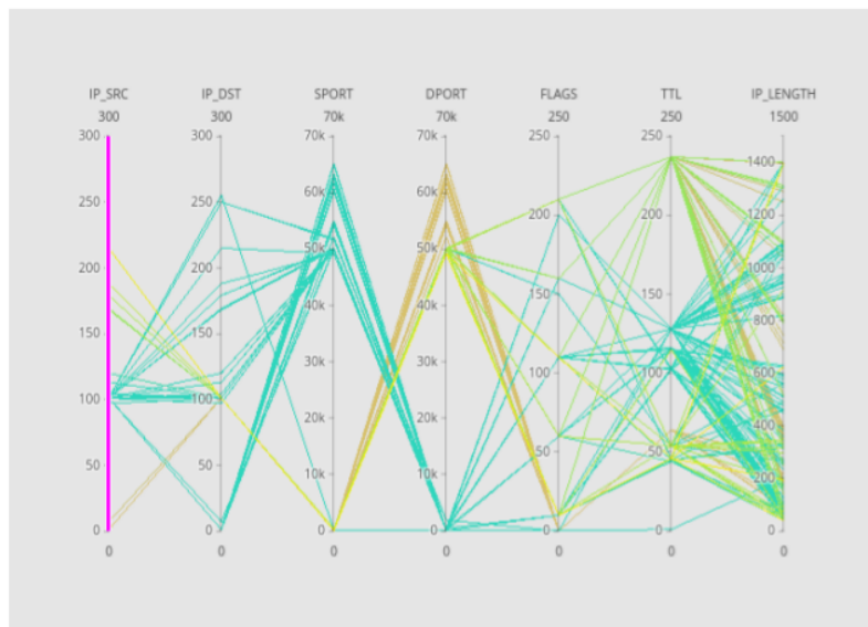
Figure 5. Gacha Traffic Pattern Visualization
