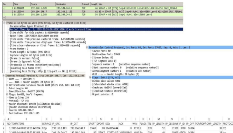
Figure 4. Screenshot of Feature Extraction Result
