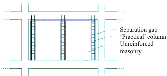
FIGURE 13. How to avoid direct contact between the brick walls and beams' and columns' main structure components (source: Charleson 2008).
