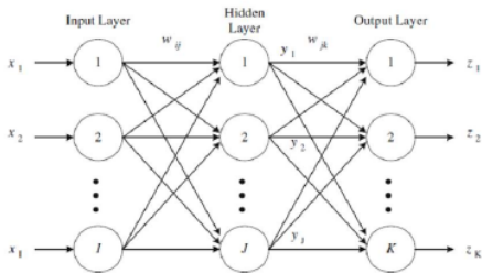
FIGURE 2.B Network Architecture backpropagation Neural Network (BNN)[16]
