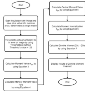
FIGURE 6. FLOWCHART EXTRACTION FEATURE GEOMETRY WITH ZERNIKE MOM
