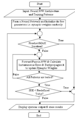
FIGURE 7. FLOWCHART BACKPROPAGATION NEURAL
