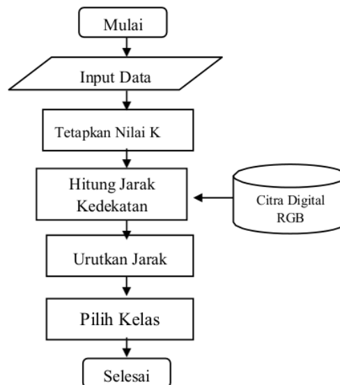
Gambar 2. Algoritma K-Nearest Neighbor
