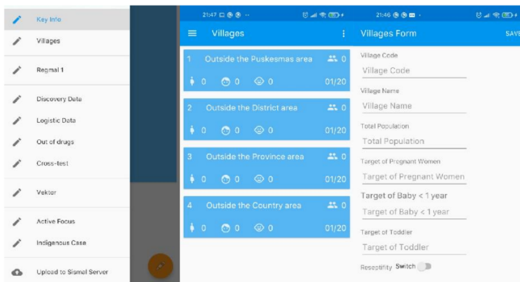
Figure 1. Application Menu
