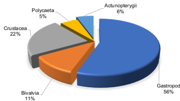
Fig. 2. Macrobenthic community structure of Musi Estuary.
