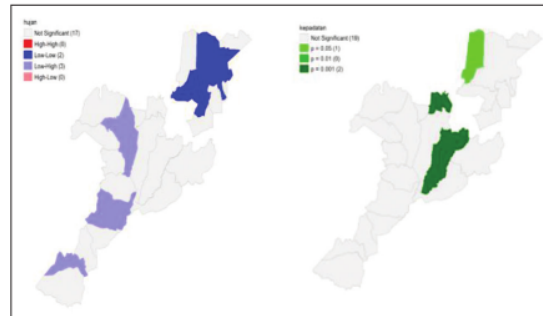
Figure 7: LISA analysis of rainfall and density variable
