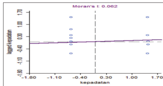
Figure 6: Moran index of rainfall and density variable
