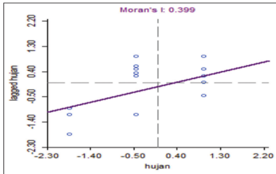
Figure 8: Moran index of rainfall and density variable
