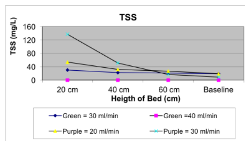
Figure 5 The effect of adsorption process on the value of TSS
