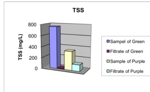
Figure 3 The effect of filtration process on TSS
