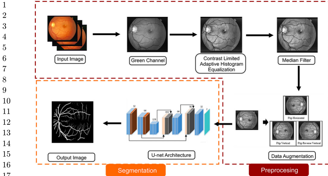
Fig. 1. Flowchart of the proposed method for data augmentation on vascular retinal image segmentation.
