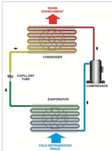
Figure 1. Refrigeration cycle
