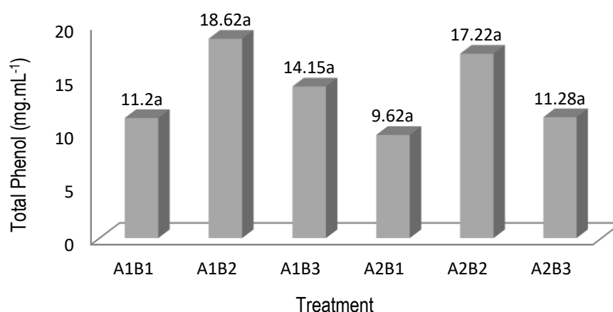
Figure 2. Total phenol ( \text{mg. mL}^{-1} ) of gaharu leaf produced by using extraction with solvents having different polarity levels.
