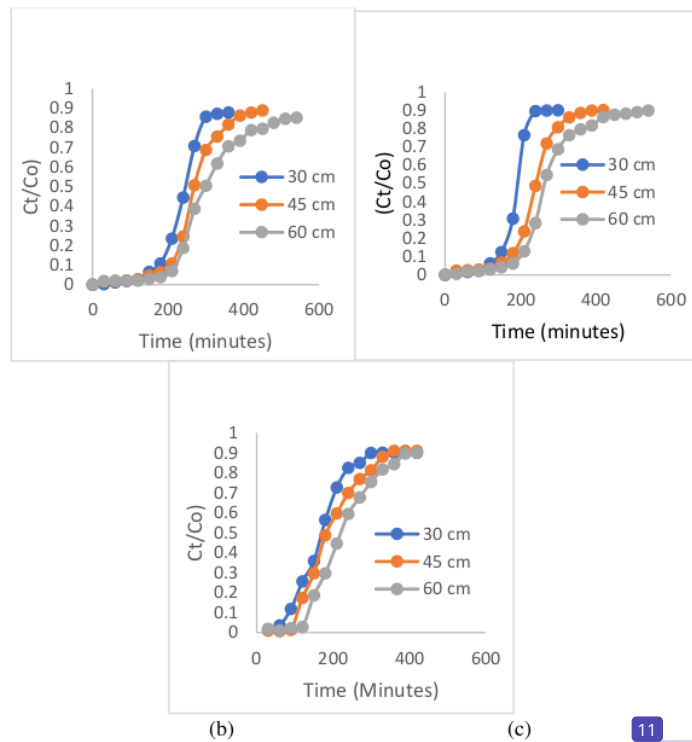
(a) Figure 7. The breakthrough curves for the ion Mn (II) at various heights bed for flow rate (a) 25 mL/min, (b) 50 mL/min, (c) 100 mL/min
