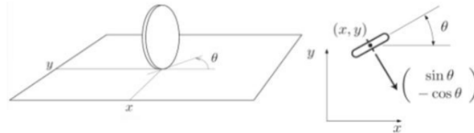
Figure 2. No lateral slip
