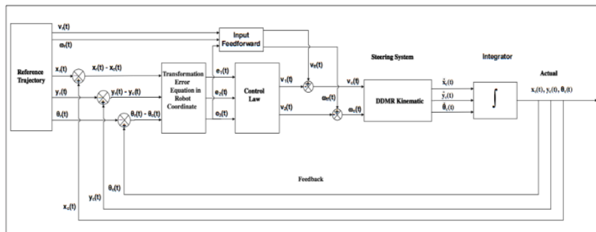
Figure 5. Block diagram control law of DDMR system
