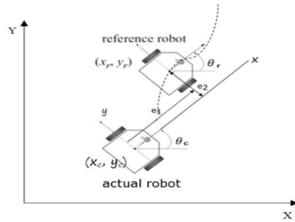
Figure 4. Transformation of error movement
