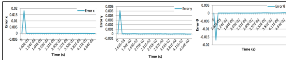
Figure 6. The DDMR error position control
