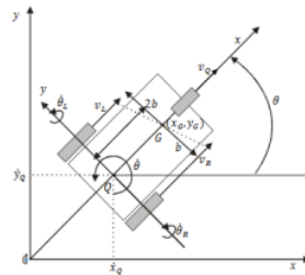
Figure 1. DDMR on 2D cartesian plane
