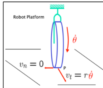
Figure 3. Pure rolling motion constraint
