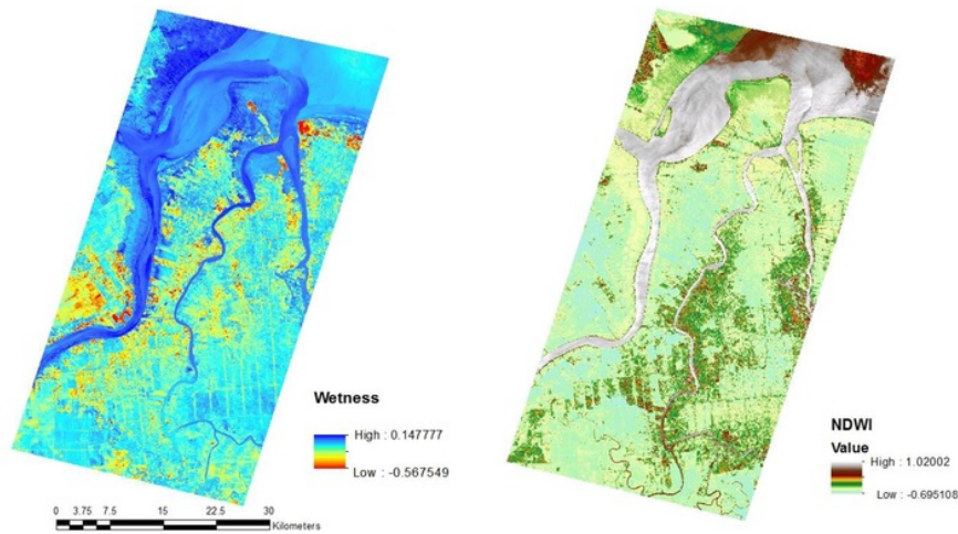
(3c) Tasseled Cap Wetness
