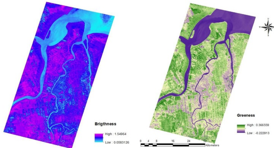
(3a) Tasseled Cap Brightness
