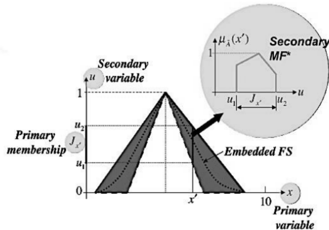
Gambar 3.6 Himpunan Fuzzy Tipe-2 (Mendel, 2009)
