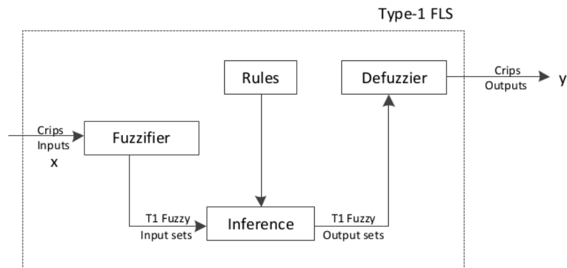
Gambar 3.1. Sistem Logika Fuzzy Tipe-1 (Mendel, 2009)
