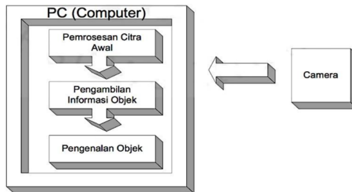
Gambar 2.2 Blok Diagram Sistem Sensor Kamera
