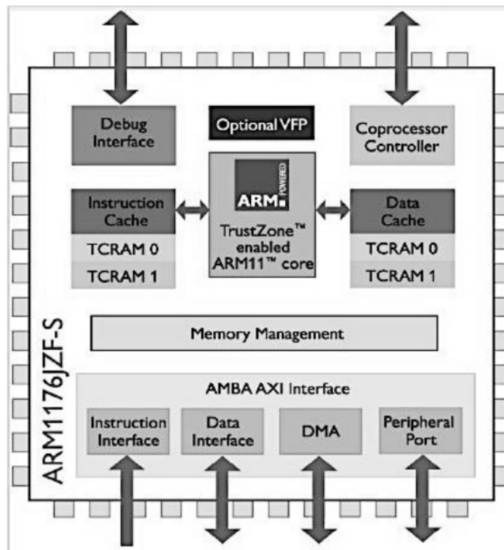
Gambar 2.3. Arsitektur Processor Broadcom BCM2835 ARM11
