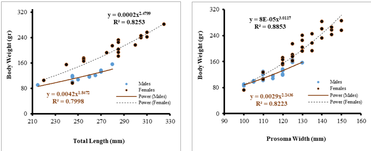
Figure 4. Total length-body weight (left) and prosoma width-body weight (right) relationship of males and females Carcinoscorpium rotundicauda from Banyuasin estuarine of South Sumatra, Indonesia. Both sex indicated the body weight grown slowly with respect to the total length (negative allometric, b < 3 , p < 0.05 ) while the body weight of females also grown slowly with respect to the prosoma width (negative allometric, b < 3 , p < 0.05 ) but the prosoma width and body weight for males grown at the same rate (isometric, b = 3 , p < 0.05 ).
