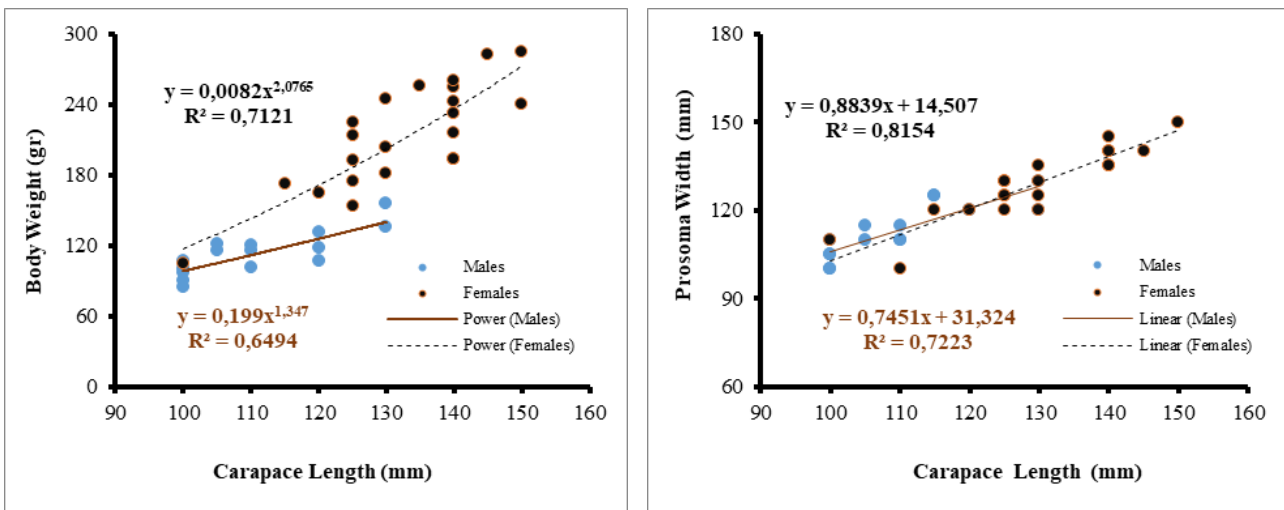
Figure 5. Carapace length-body weight (left) and prosoma width-carapace length (right) relationship of males and females Carcinoscorpium rotundicauda from Banyuasin estuarine of South Sumatra, Indonesia. The body weight grew slowly with respect to the carapace length (negative allometric, b < 3 , p < 0.05 ) for both sexes while the carapace length and prosoma width grown at the same rate (isometric, b = 1 , p < 0.05 ).
