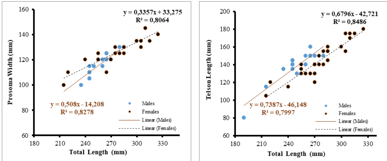
Figure 6. Prosoma width-total length (left) and telson length-total length (right) relationship of males and females Carcinoscorpius rotundicauda from Banyuasin estuarine of South Sumatra, Indonesia. The telson length or prosoma width grew slowly with respect to the total length (negative allometric, b < 1 , p < 0.05 ) for both sexes.
