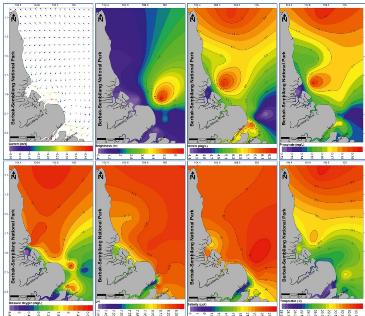
Fig. 2. Physicochemical parameters in Banyuasın water.
