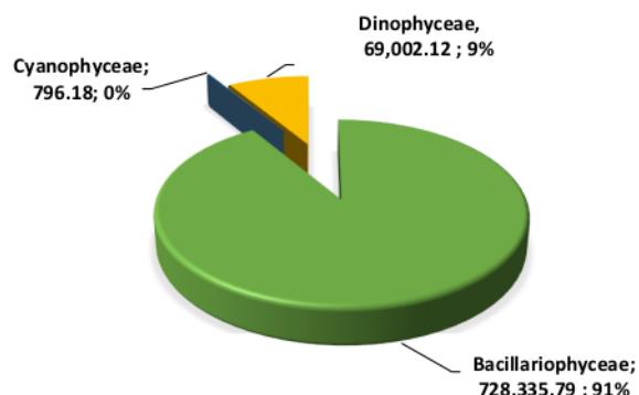
Fig. 3. Phytoplankton community structure in Banyuasın water.
