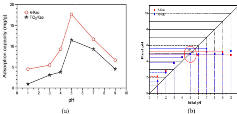
Figure 5. Effect of initial pH (a), and pH point zero charge ( pH_{pzc} ) of activated kaolin and TiO 2 /Kaolin composite (b).
