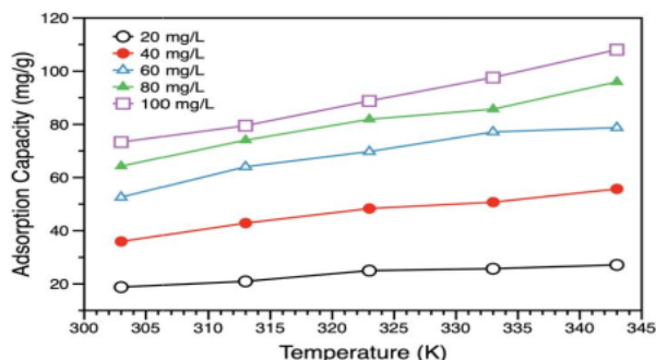
Figure 6. Effect of temperature on the adsorption capacity.
