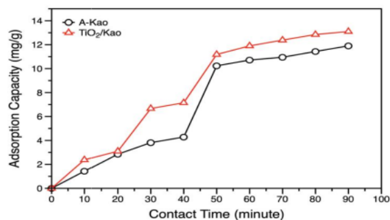
Figure 4. Effect of contact time on the adsorption performance.
