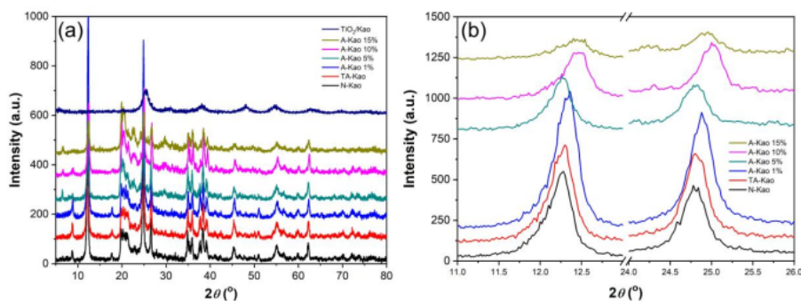
Figure 2. XRD pattern: (a) natural kaolin, activated kaolin, and TiO 2 /Kaolin composite and (b) the change of the main characteristic of the kaolin reflection peak at 2\theta around 12° and 25° due to the activation process.
