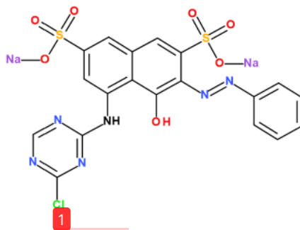
Figure 1. Chemical structure of Procion red.
