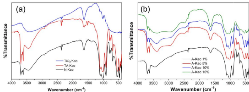
Figure 3. FTIR spectra of (a) natural kaolin, thermal activated kaolin, \text{TiO}_2 /Kaolin composite and (b) acid-activated kaolin at the different acid concentration.
