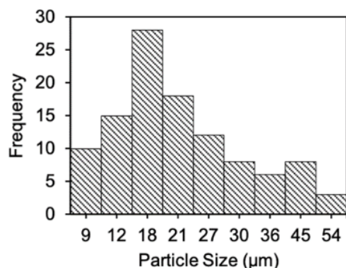
Figure 5. Distribution of particles size of CuAl/BC composite.
