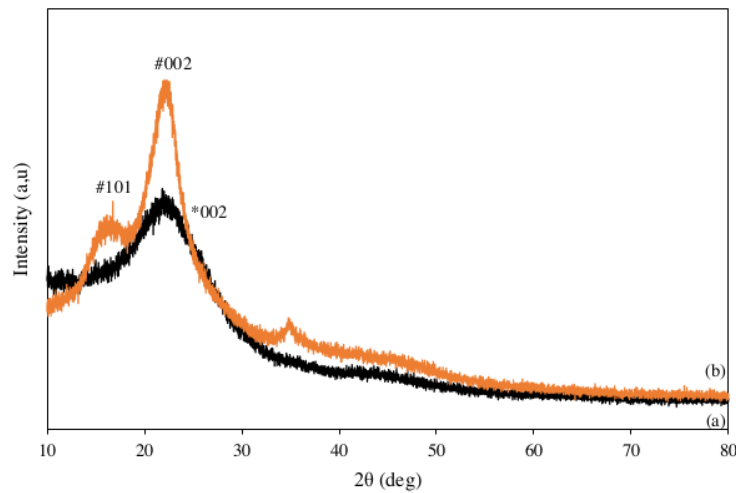
10 Figure 1. XRD powder patterns of (a) RH-BC and (b) RH
