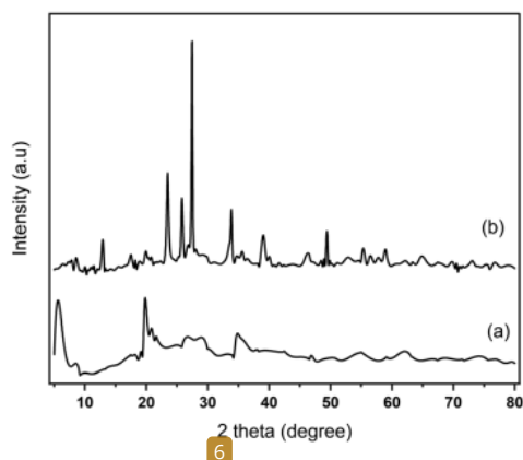
Fig. 1 Diffractograms of (a) Na-bentonite and (b) MoN-bentonite.
