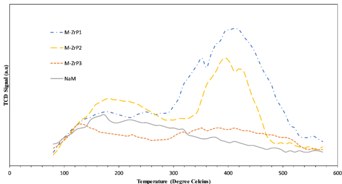
Fig. 4 NH 3 -TPD of catalysts
