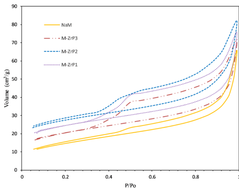
Fig. 3 N 2 adsorption-desorption of catalysts
