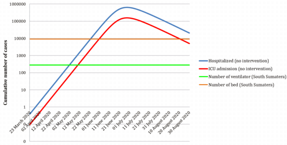
Fig. 9 Prediction of the number of cases that need hospital treatment for the availability of ventilators and beds in South Sumatera Province
