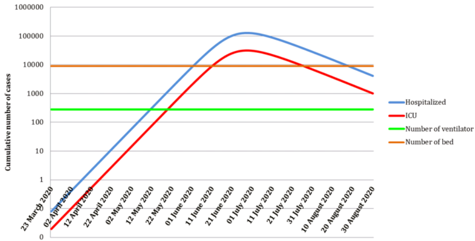
Fig. 10 Prediction of the number of cases that need hospitalization for the availability of ventilators and beds with multiple interventions
