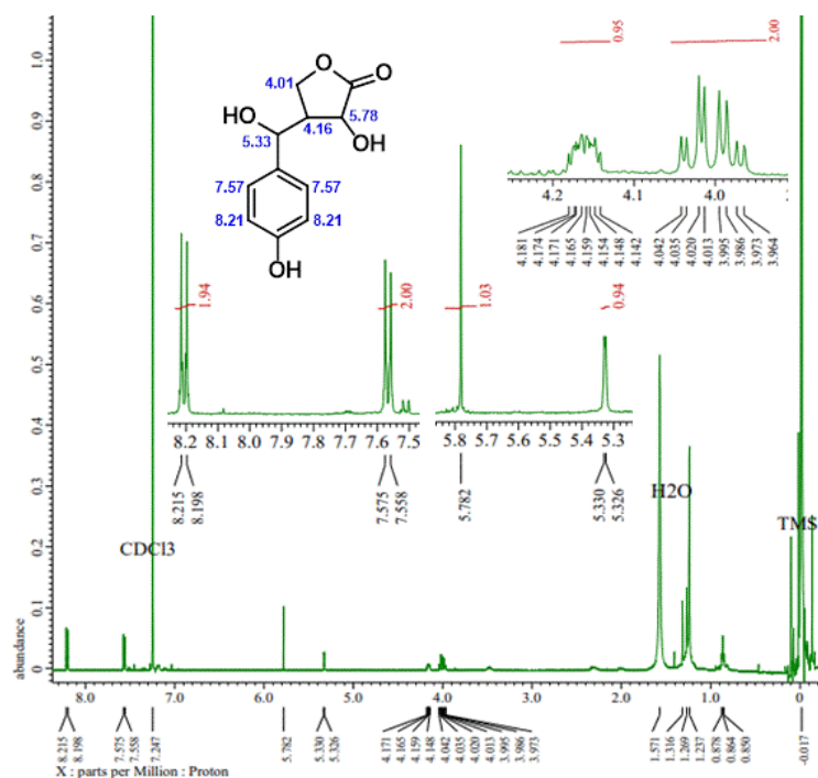
Figure 4. The ^1\text{H} -NMR spectrum of compound 1
