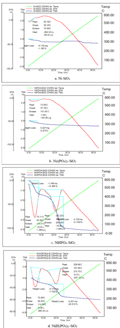
Figure 2. TGA-DTA graph of pyridine adsorbed nickel phosphate catalysts a) Ni-SiO 2 b) Ni 3 (PO 4 ) 2 -SiO 2 c) NiHPO 4 -SiO 2 d) Ni(H 2 PO 4 ) 2 -SiO 2
