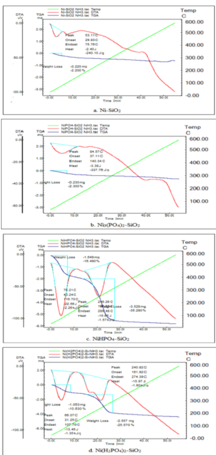
Figure 1. TGA-DTA from ammonia adsorbed Nickel phosphate catalyst a) Ni-SiO 2 b) Ni 3 (PO 4 ) 2 -SiO 2 c) NiHPO 4 -SiO 2 d) Ni(H 2 PO 4 ) 2 -SiO 2
