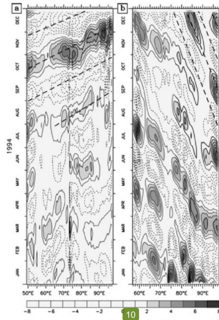
Figure 5 Same as Figure 4 except for the period of January – December 1994.
