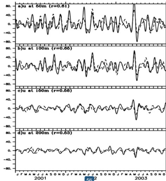
Figure 1 (a) 200-day band-passed time series of the observed (solid) and model (dashed) zonal currents (cm/s) in the eastern equatorial Indian Ocean ( 0^{\circ}\text{N} , 90^{\circ}\text{E} ) during January 2001 – December 2003 at 50-m depth. (b)-(d) Same as (a) except for currents at 100-m, 150-m and 200-m depth, respectively.
