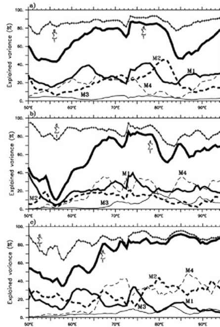
2 Figure 6 (a) Explained variance along the equator referenced to the 70-100-day band-passed pressure for mode 1 contribution (thick line), mode 2 (thick dashed line), mode 3 (thin line), mode 4 (thin dashed line), sum of the first four modes (extra thick line) and sum of the first six modes (crossed line). The vertical mode decomposition is based on the mean density profiles for January 1999 – December 2000. For (b) and (c) same as in (a) except for the mean density of September 1997 – March 1998 and July – December 1994, respectively.
