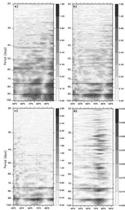
11 Figure 2 Variance-preserving spectra of (a) observed sea surface height from TOPEX/Poseidon ( \text{cm}^2 ), (b) model sea level ( \text{cm}^2 ), (c) modeled depth of 20^\circ\text{C} isotherm ( \text{m}^2 ) and (d) observed zonal wind stress ( \text{dyn}^2 \text{cm}^{-4} ) along the equatorial Indian Ocean (averaged over 1^\circ\text{S} - 1^\circ\text{N} ). The spectra were calculated based on a 10-year record (1993-2002) from TOPEX/Poseidon and a 14-year period (1990-2003) for other fields.
