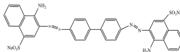
Figure 1. Structure Congo Red.
