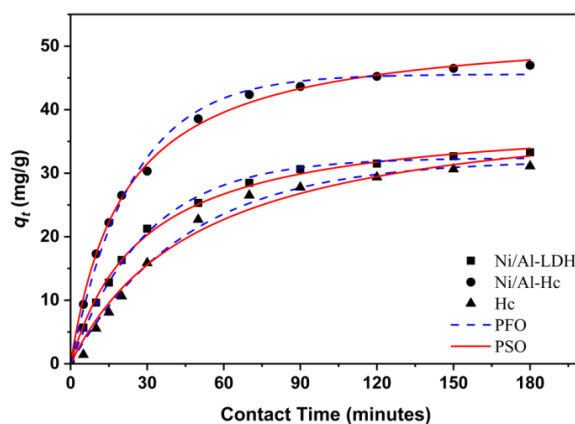
Figure 8. Kinetic models of Ni/Al, Hc, and Ni/Al-Hc.
