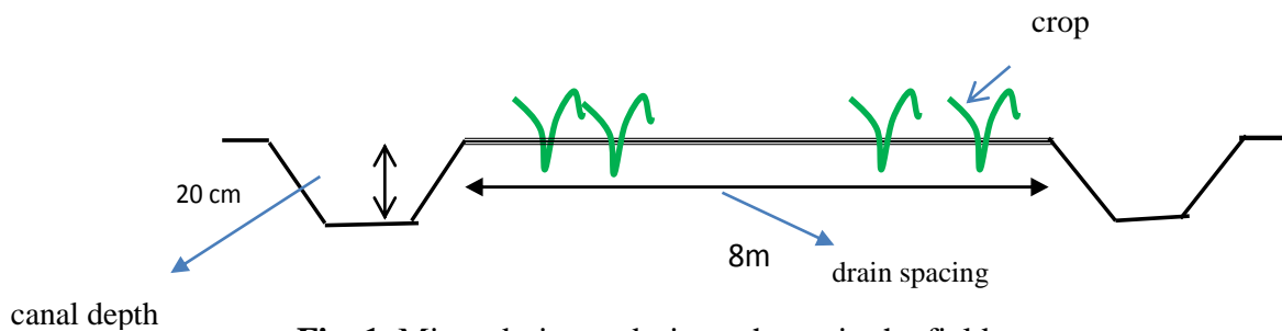
Fig. 1. Micro drainage design scheme in the fields
