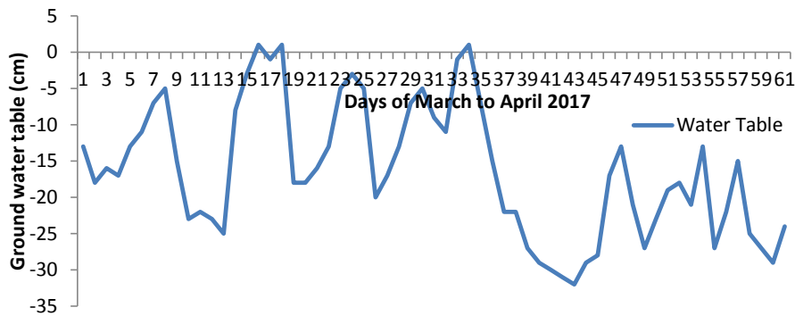
Fig 7. The daily water table fluctuation in the field
