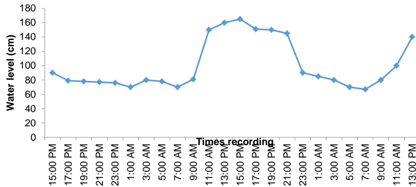
Fig. 5. Fluctuations of surface water in secondary channel in the Mulyasari village
