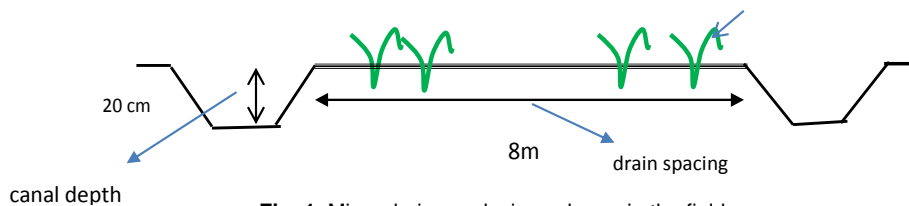
Fig. 1. Micro drainage design scheme in the fields
