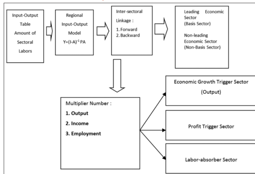
Graph 2: Research Framework
