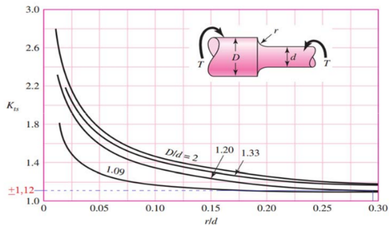
Gambar 1. Peterson Factors for Stress Concentration ( K_t )
