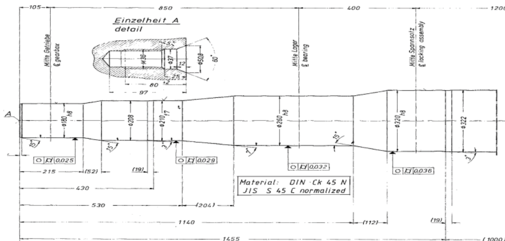
Gambar 2. Desain shaft drive pulley
