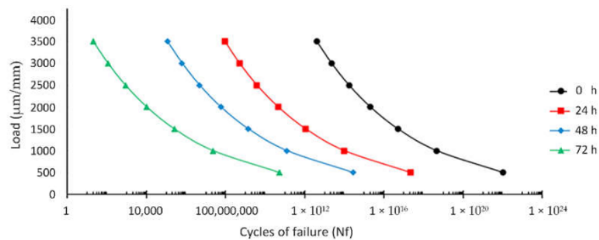
Figure 4. Load ( \mu\text{m}/\text{mm} ) vs Cycles of failure (Nf).
