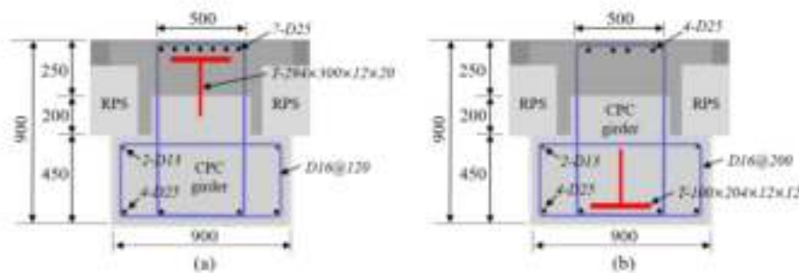
Figure 5. Section design for CPC girder: (a) Detail at both ends; (b) detail at mid-section.
