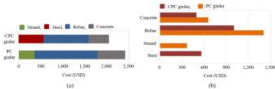
Figure 7. Cost proportion and comparison of a typical girder: (a) Cost proportion; (b) cost comparison.
