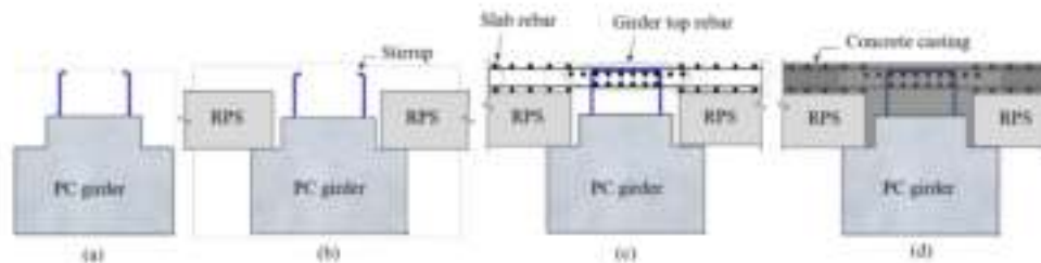
Figure 3. Construction process of the precast concrete (PC) frame: (a) PC girder installation; (b) rib-plus precast concrete slab (RPS) installation; (c) slab and girder rebar placement; (d) concrete casting.
