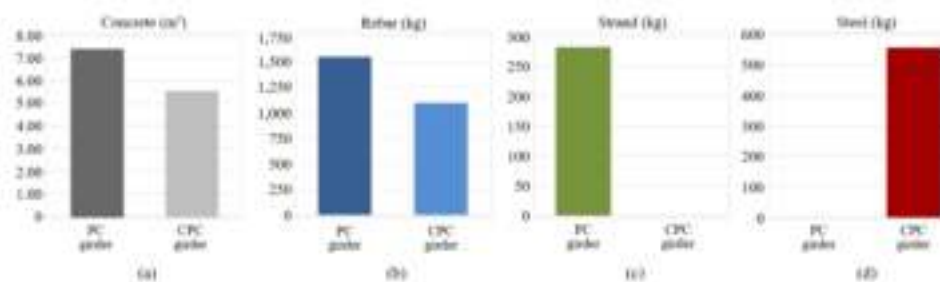
Figure 6. Quantity of resources for each PC and CPC girder: (a) concrete; (b) rebar; (c) strand; (d) steel.
