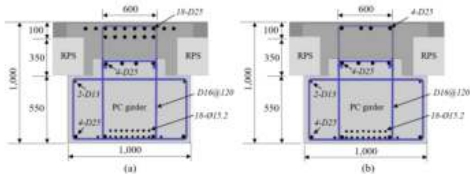
Figure 4. Section design for typical PC girder: (a) Detail at both ends; (b) detail at mid-section.
