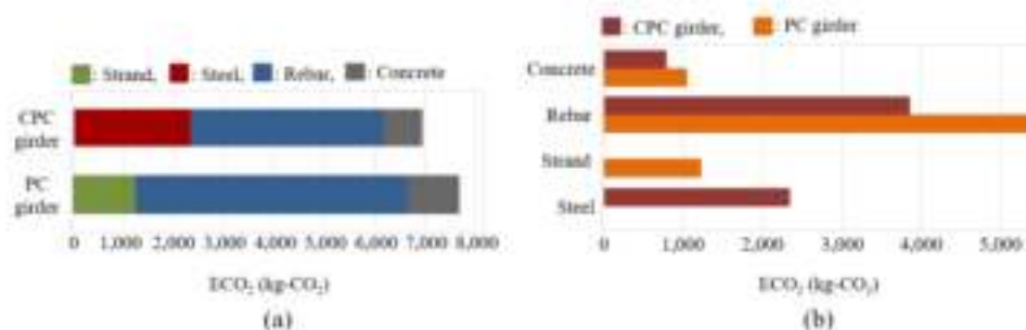
Figure 8. ECO 2 proportion and comparison of a typical girder: (a) ECO 2 proportion; (b) ECO 2 comparison.
