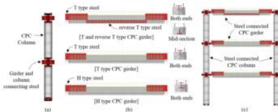
Figure 1. Overview of the SMART (Sustainable, Measurable, Attainable, Reliable, and Timely) frame: (a) Steel connected composite precast concrete (CPC) column; (b) CPC girders; (c) typical SMART frame with three types of girder.
